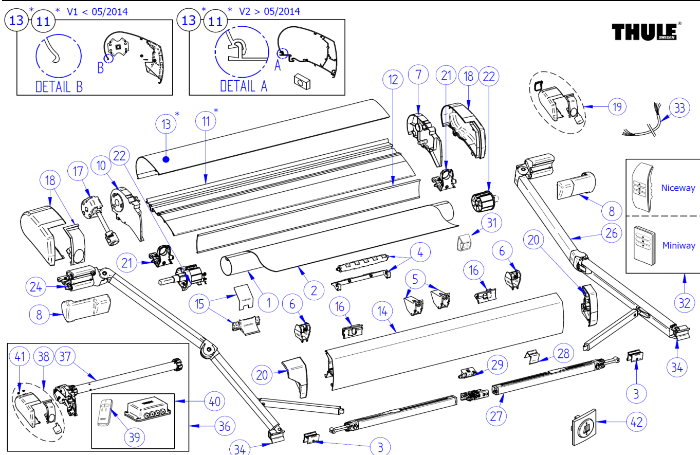
THULE Omnistor 9200
